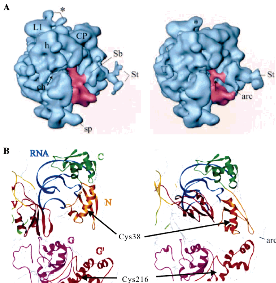
FIGURE 1: G \rightarrow L11-NTD movement. (Left) Complex 1, 70S·EF-G·GDP·CP; (right) complex 2, 70S·(tRNA) 2 ·EF-G·GDP·FA (adapted from ref 10). (A) Entire 70S ribosome. The position of bound EF-G is indicated in red. Landmarks of the 50 S subunit: L1, protein L1; St, stalk; Sb, stalk base; arc, arc-like connection. Landmarks of the 30 S subunit: h, head; sp, spur; ch, mRNA channel. (B) Detail showing N-terminal (N) and C-terminal (C) portions of L11 and G and G' regions of EF-G. The positions of L11 residue 38 and EF-G residue 216 are indicated. The position and inferred conformation of EF-G are the same when tRNA is omitted from complex 2 (9).
